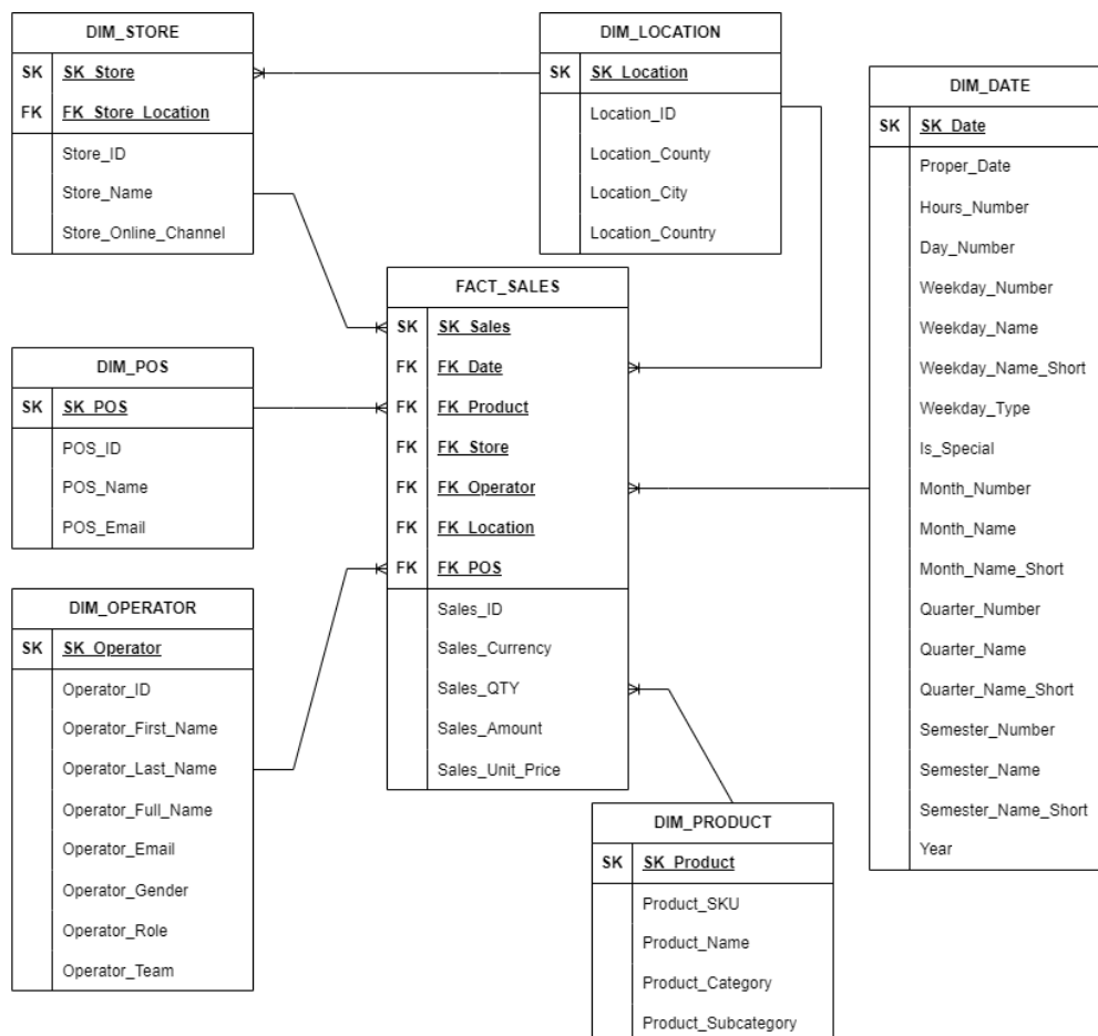
Figure 2: Start Schema
